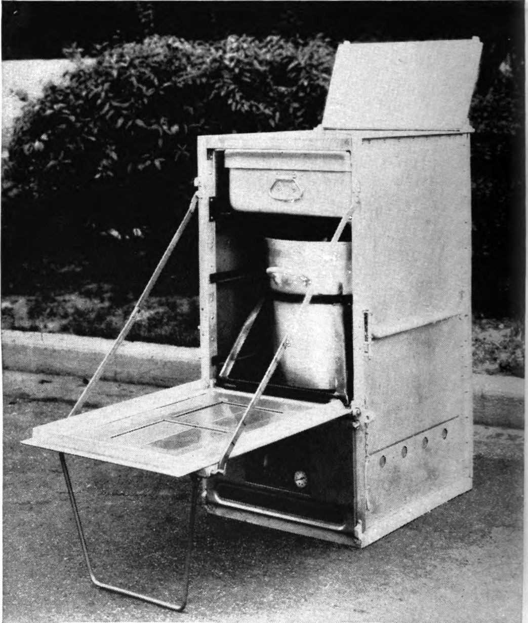
FIGURE 30.—One unit of range with cooking equipment in place.
